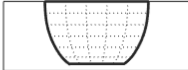
Lat [-90 0], Lon [-180 -30]
