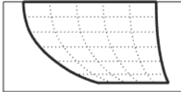
Lat [-90 0], Lon [-180 -30]
