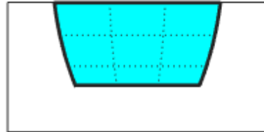
Lat [-70 -30], Lon [60 150]
